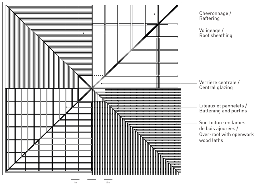
Plan de charpente secondaire / Plan of the secondary framing
